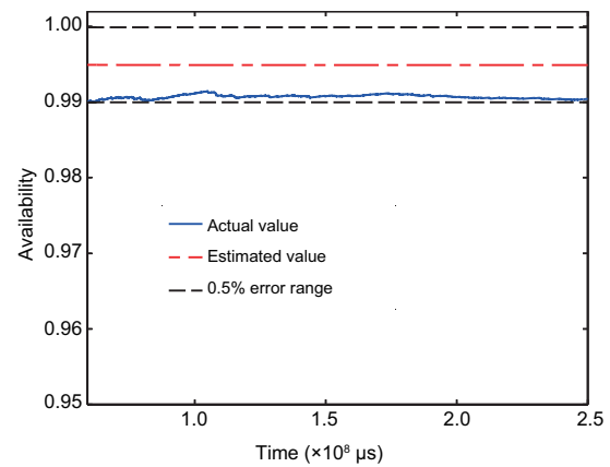
Fig. 13 Comparing the estimated and actual values of \mathcal{A} in a nine-node network when \lambda_{A(t)} = 1000 faults/s
